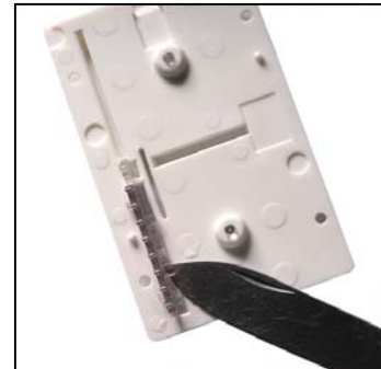
Snap out the light pipes with a flat tool
