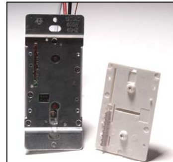
Paddle Assembly and SwitchLinc body separated
